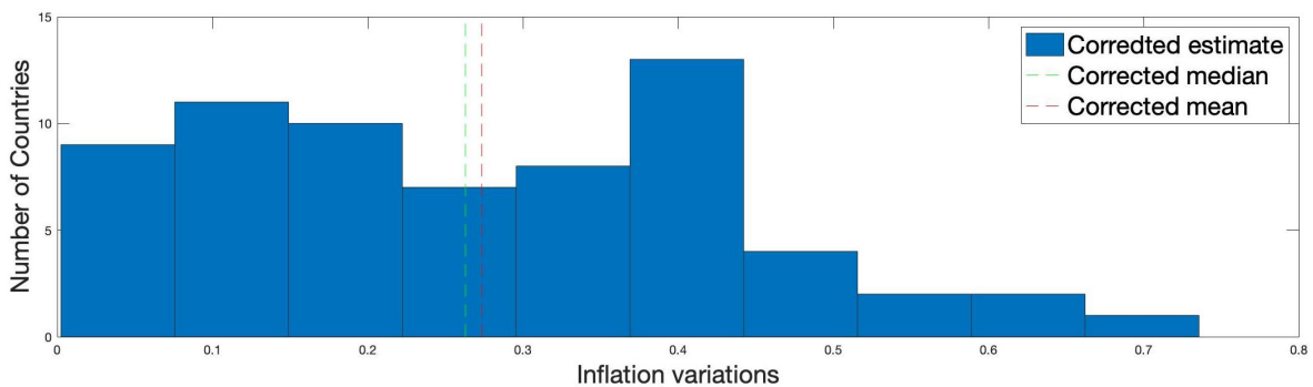
Fig. 3: The frequency distribution of the fraction of variance explained by the commodity price factors, over the period 1970-2014.
